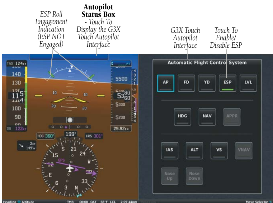
AFCS (ESP Enabled)
