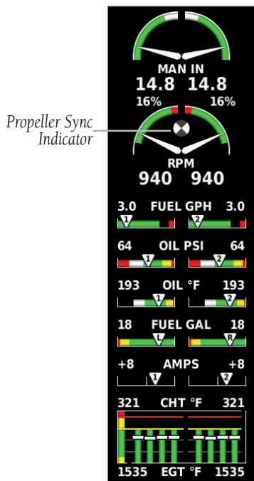
Example Engine Indication System (PFID) (Multi-Engine)
