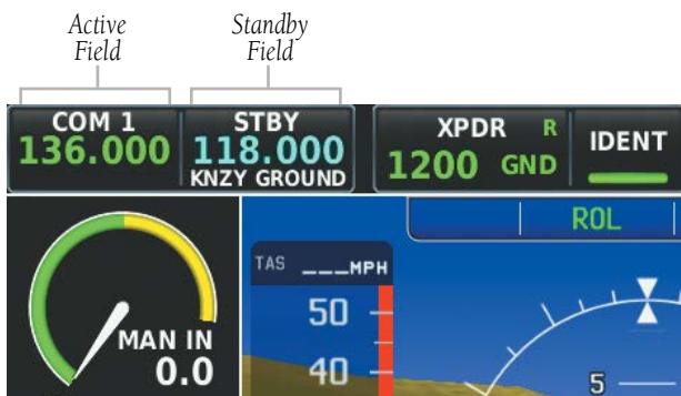
COM Radio on PFD
