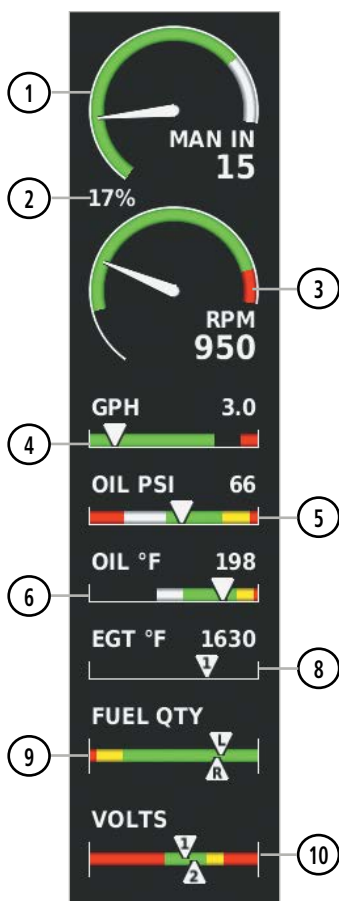
Example Engine Indication System (PFD)
