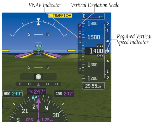
VNAV Indications (PFD)
