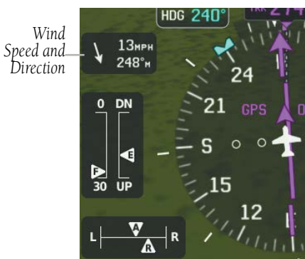
Wind Data
